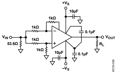
Figure 42. Common-Mode Rejection
