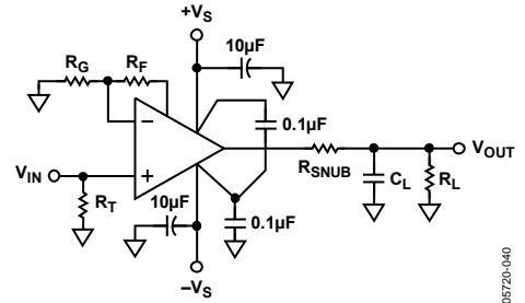
Figure 43. Typical Capacitive Load Configuration
